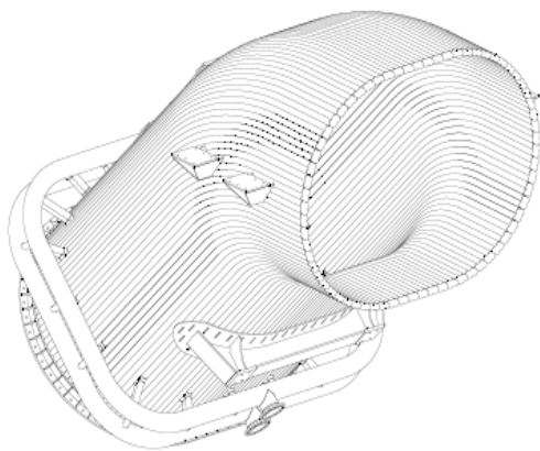
Figure 7: Water cooled part of the offgas duct of an EAF
