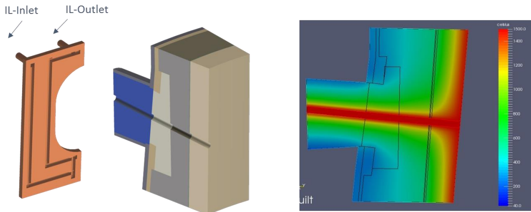
Figure 5: Special design of the cooled tap hole with the copper cooled back plate mounted upon the steel shell (left and middle) and CFD modelling of the temperature distribution during the taping of hot metal
