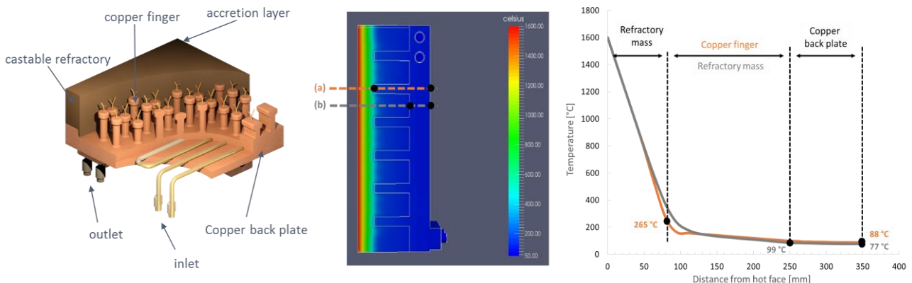
Figure 2: Special design of a composite furnace module cooling (CFM) element for creating a freeze lining (left) and CFD modelling of the temperature distribution at a furnace temperature of 1600°C (middle) and resulting steep temperature gradient within the refractory mass (right)
