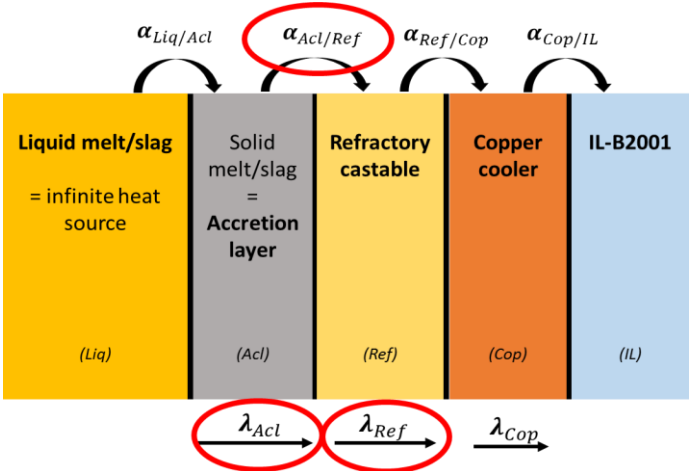
Figure 1: Schematic picture of the different layers within the entire system in industrial scale use within a copper cooling element
