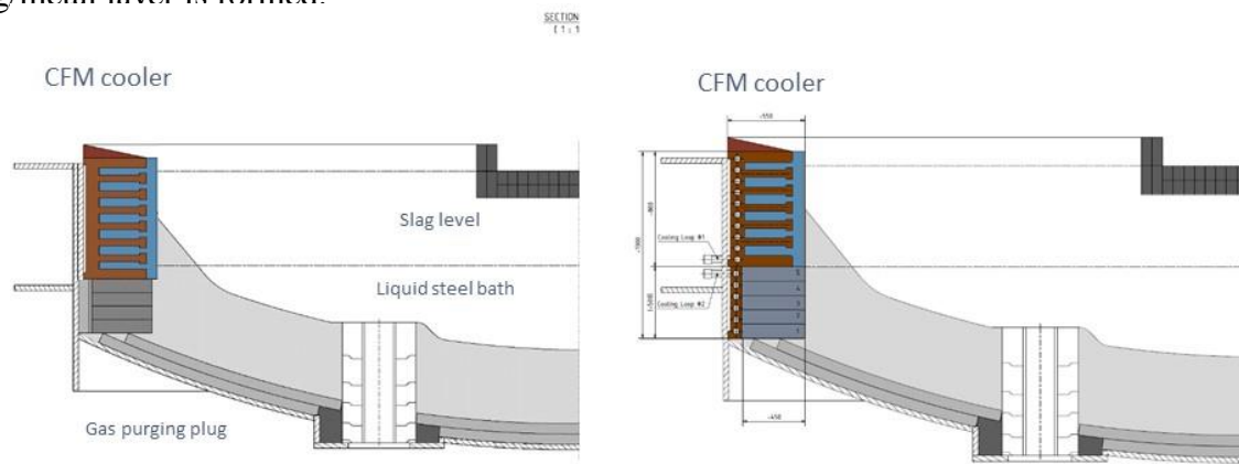
Figure 6: Different opportunities for installation of an high intensity cooler within the side wall of an EAF, left: installation of the cooler only at the slag line; right: slag line cooling with CFM elements and cooled copper plate behind the brick lining at the lower part
